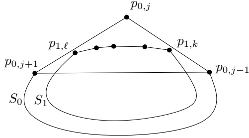
Fig. 1. Removing a point p_{0,j} from S_0 exposes a chain p_{1,\ell}, \dots, p_{1,k} of S_1 .
